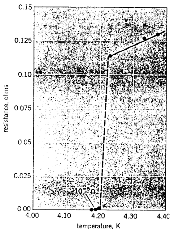
Fig. 1. Resistance in ohms of a specimen of mercury versus absolute temperature. ^{\circ}\text{F} = (\text{K} \times 1.8) - 459.67 . (After H. Kamerlingh Onnes, Akad. van Wetenschappen, Amsterdam, 14:113, 818, 1911)
